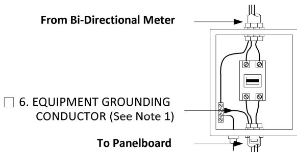
Figure 1 - RE SYSTEM VISIBLE DISCONNECT DEVICE
