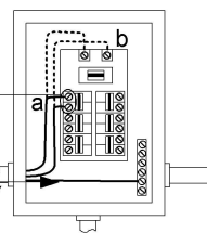
Figure 2 - PANELBOARD / SERVICE EQUIPMENT
