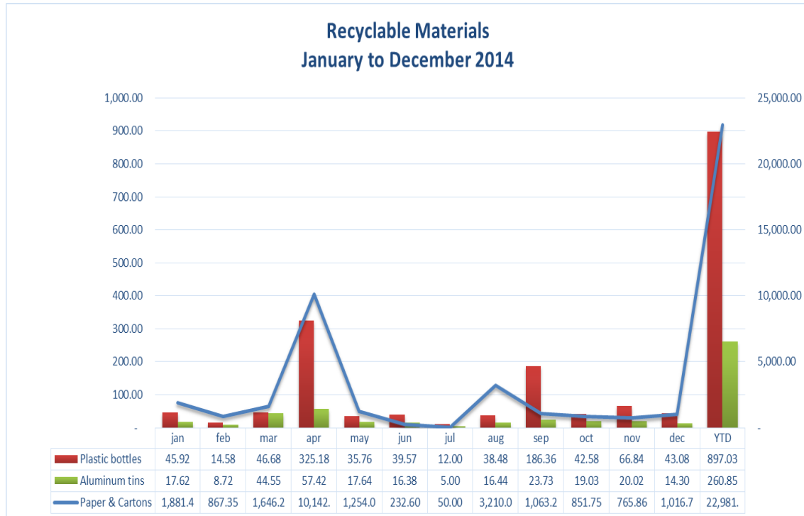
Figure 6: 2014 Recyclable Materials
