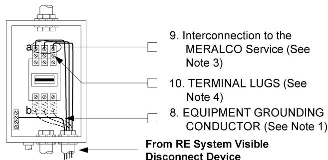
Figure 3. SERVICE EQUIPMENT
