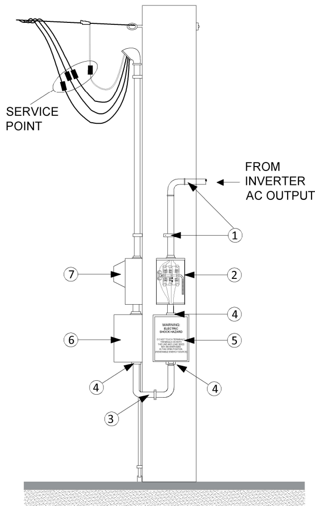
Figure 2. RE SYSTEM VISIBLE DISCONNECT DEVICE
